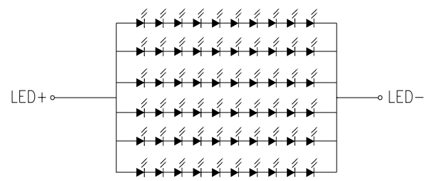
BACKLIGHT CIRCUIT DIAGRAM
